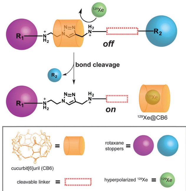
Scheme 1 General strategy for activating CB6-rotaxanes for ^{129}\text{Xe} NMR. A rotaxane with a triazole-diammonium-CB6 center and a cleavable linker blocks ^{129}\text{Xe} -CB6 interactions and thus suppresses ^{129}\text{Xe@CB6} NMR signals. Once cleaved, the CB6 ring can dissociate and serve as a host for hyperpolarized ^{129}\text{Xe} , producing a ^{129}\text{Xe@CB6} NMR signal.
