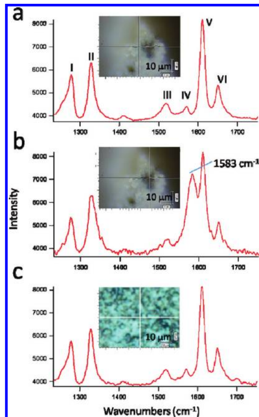
Figure 6. Raman spectra with optical insets of (a) a PPTA region within the p -MWNTs/PPTA composite, (b) an aggregate of p -MWNTs within the p -MWNTs/PPTA composite, (c) a representative area of the PPTA-MWNT/PPTA composite.
