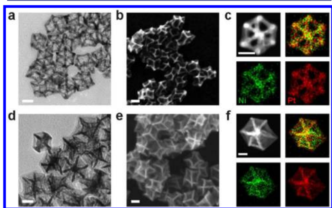
Figure 2. TEM and SEM images of (a, b) hollow nanoframe and (d, e) excavated nanoframe (scale bars represent 20 nm). STEM-HAADF image and STEM-EDS mapping of (c) hollow nanoframe and (f) excavated nanoframe oriented in the <111> direction (scale bars represent 10 nm).
